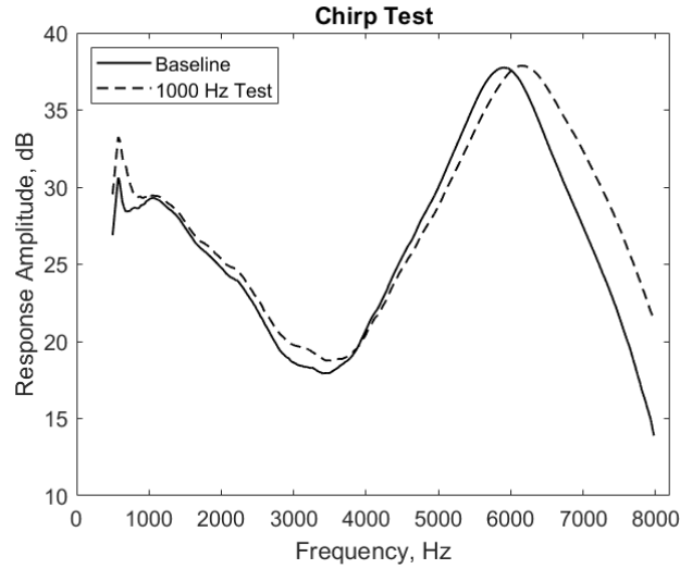
Figure 15: Chirp frequency response example
